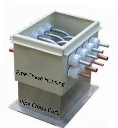
Top view of the "Medium" Pipe Chase Housing with the lid removed with 16 Sigrist Exit Seals® installed
